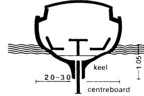
17 Centreboard keel cruiser: section
